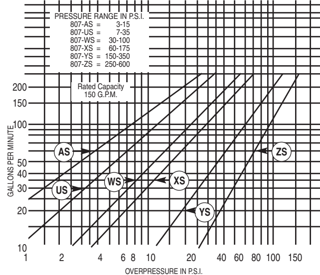
2" VALVE TESTS
