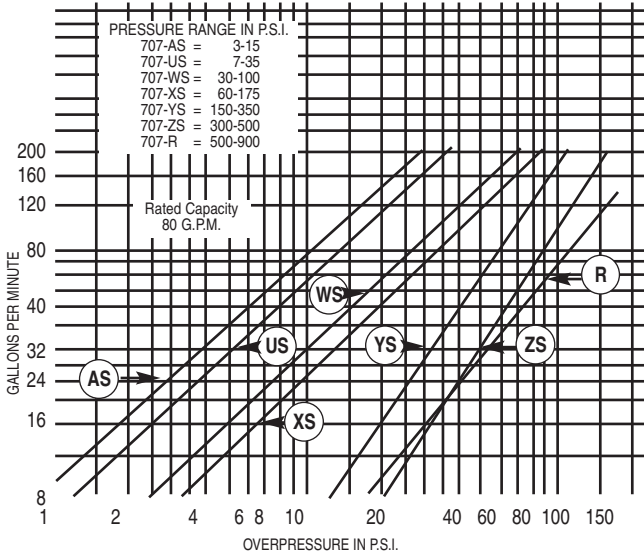
1 1/2" VALVE TESTS
