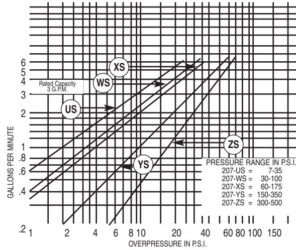
3/8" VALVE TESTS
